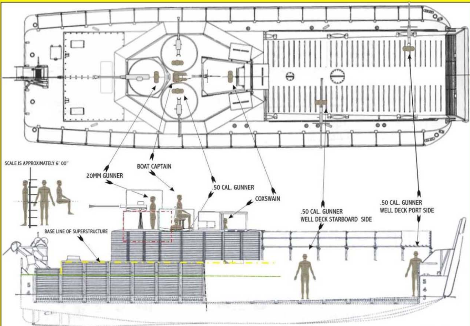
ARMORED TROOP CARRIER (ATC) - CREW MEMBER'S AT BATTLE STATIONS
