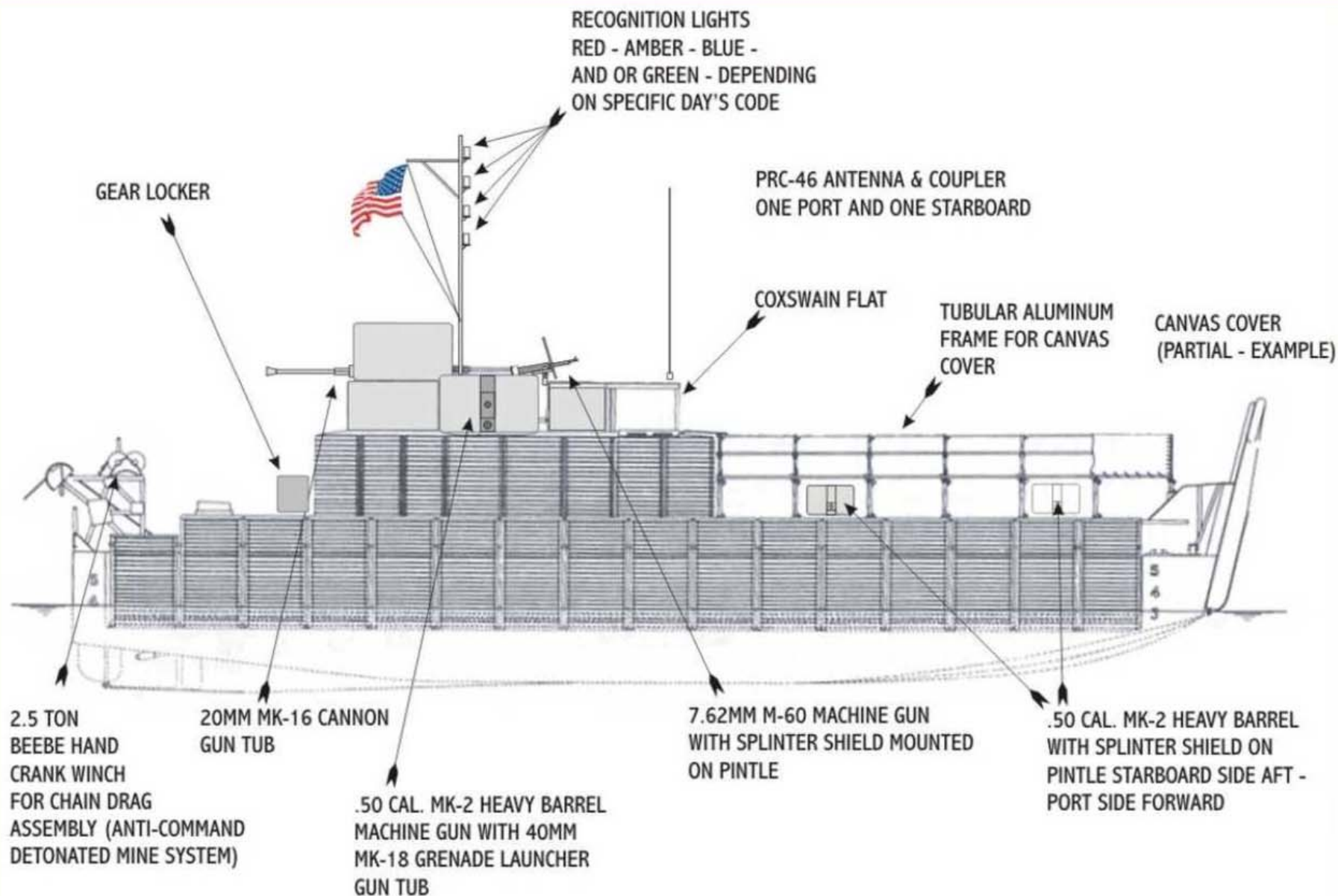
ARMORED TROOP CARRIER (ATC) - "RAG TOP" - EMPTY WELL DECK
