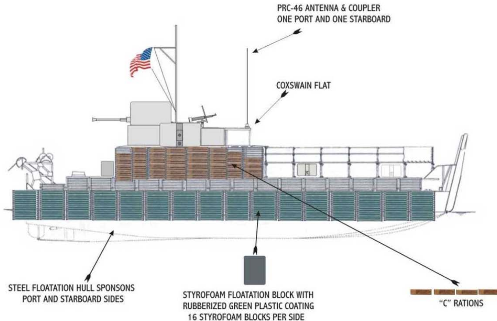
ARMORED TROOP CARRIER (ATC) - "RAG TOP" - EMPTY WELL DECK
